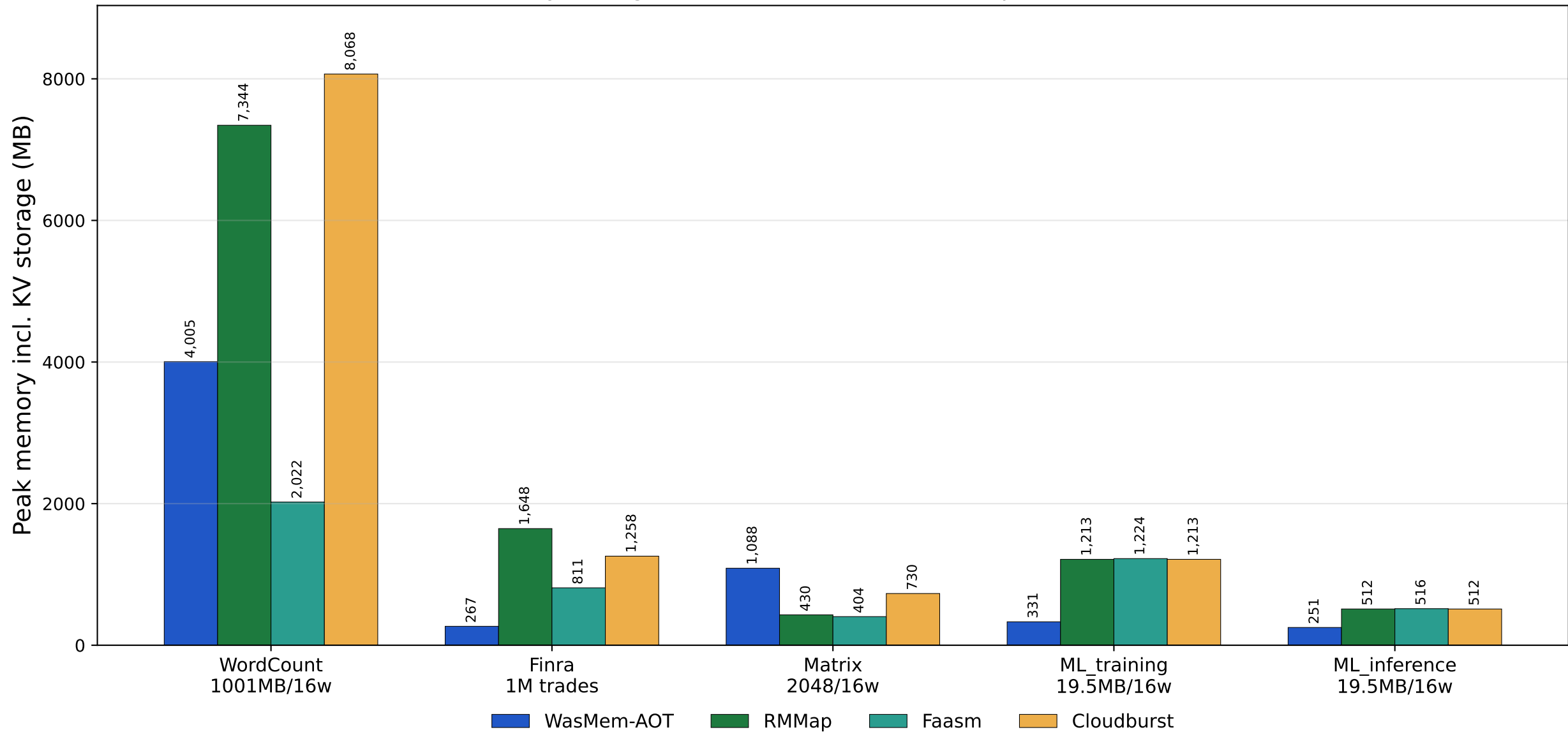
Peak memory at largest load — WasMem vs RMMMap / Faasm / Cloudburst
